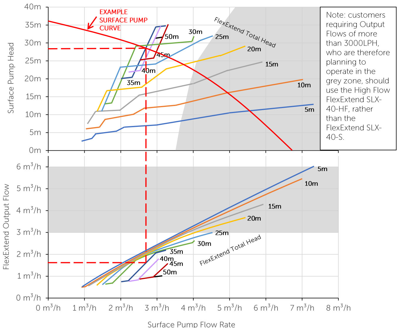
SLX-40-S surface drive pump selection
